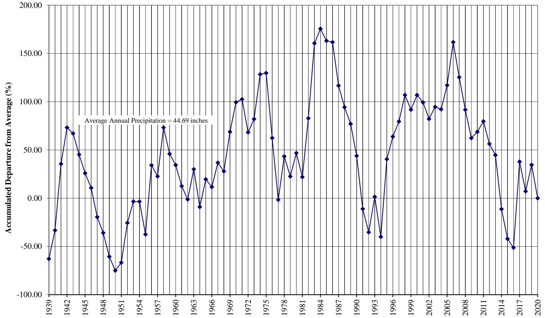
FIGURE 1 Hidden Valley Lake Community Services District Accumulated Departure from Average Annual Precipitation Measured at the Middletown Station (1,2) Water Years 1939 - 2020
